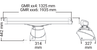
GMR XHD2 SERIES
