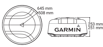
GMR DOME SERIES
