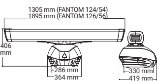
GMR FANTOM SERIES
